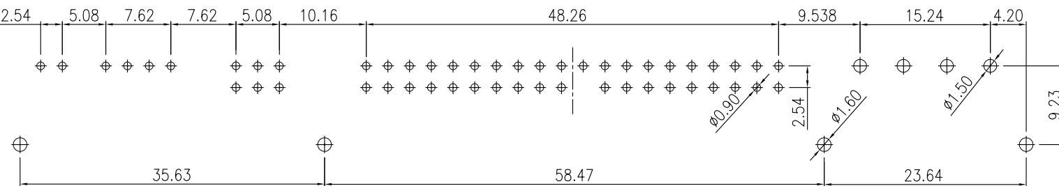
PC BOARD LAYOUT
