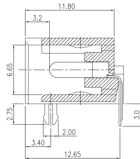
SEC A-A SCALE 3/1
